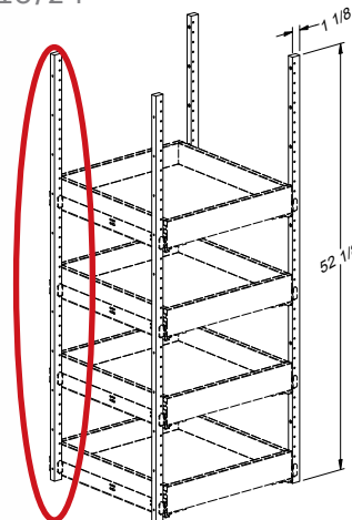
Tall Cabinets SST_PK4
